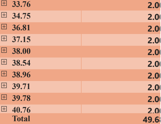
response_time_hours AvgRecoveryDuration
