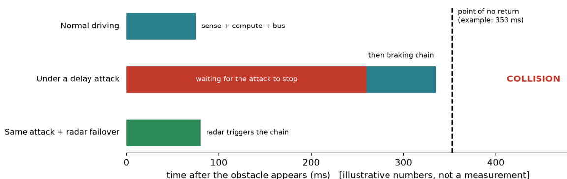
Figure 2. Why timing matters (illustrative numbers). A delay attack pushes the brake past the point of no return; a second, independent sensor lets the chain start without waiting.
