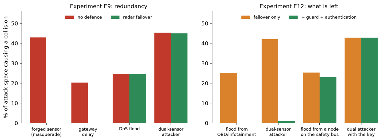
Figure 3. Measured results (hazard volume = share of the attack space that causes a collision). Left: radar failover. Right: after adding the gateway guard and authentication.
