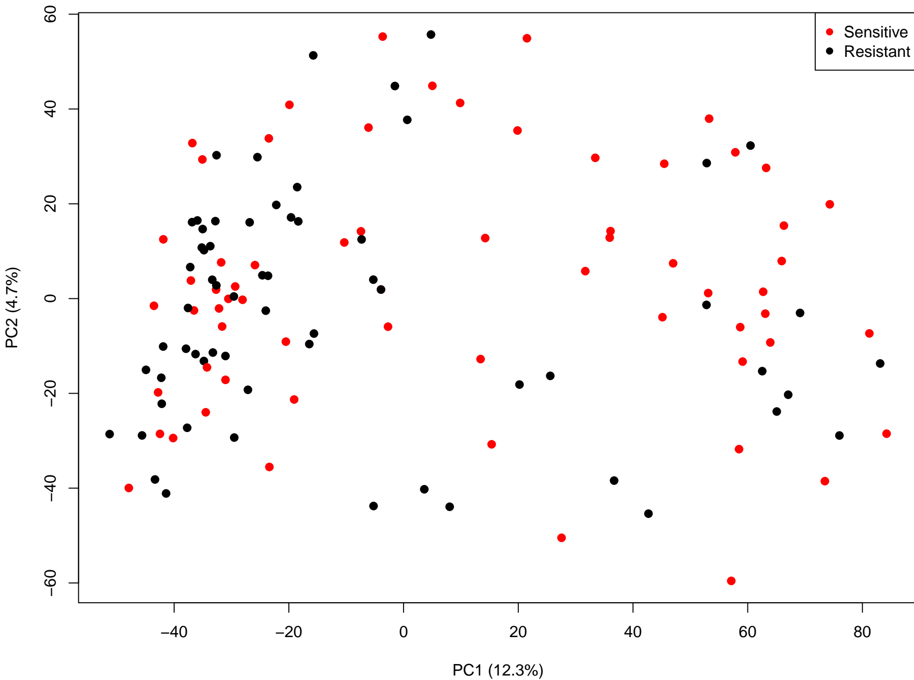
PCA: Lung Cancer Cisplatin Response
