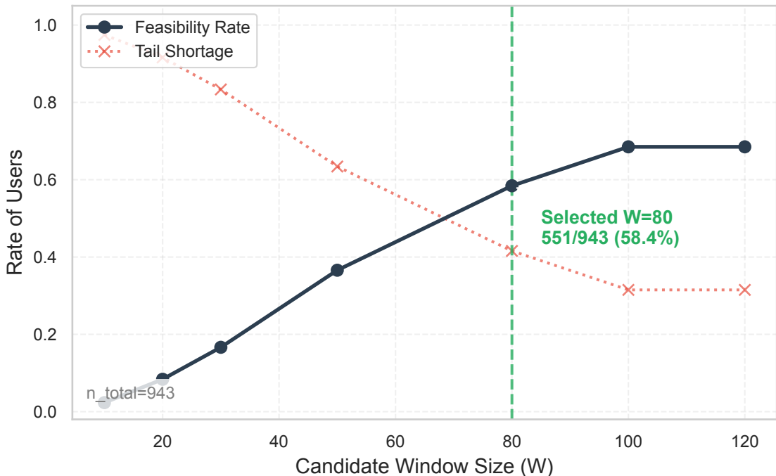
Constraint Feasibility vs. Window Size
