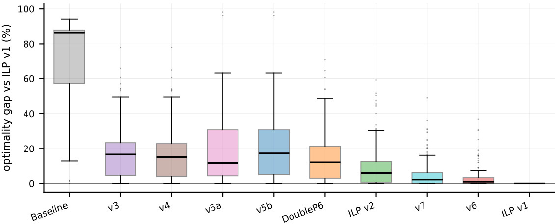
Per-instance gap distribution (220 instances, no averaging)
