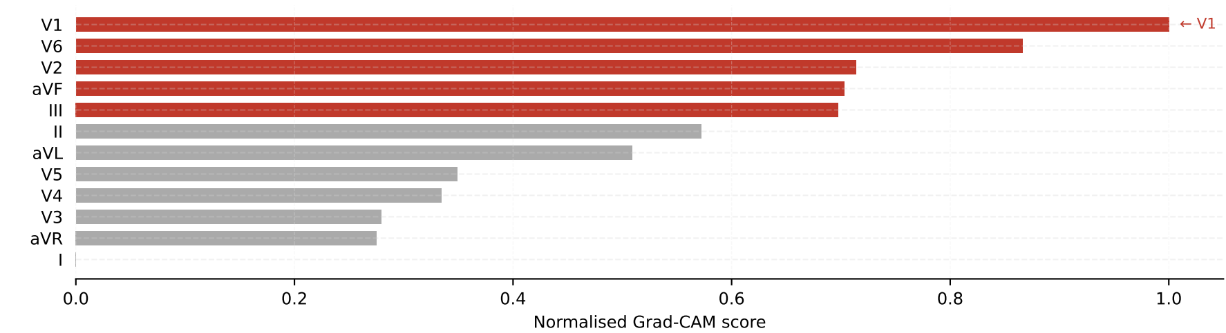
B Activation per lead
