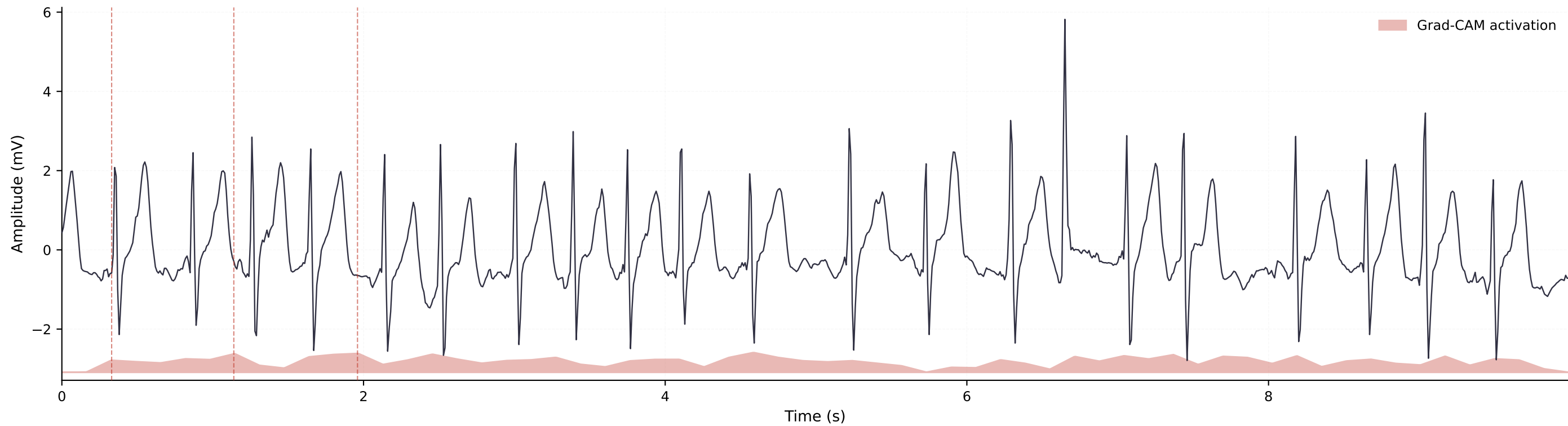
A Grad-CAM explanation — AFIB (Lead I)
