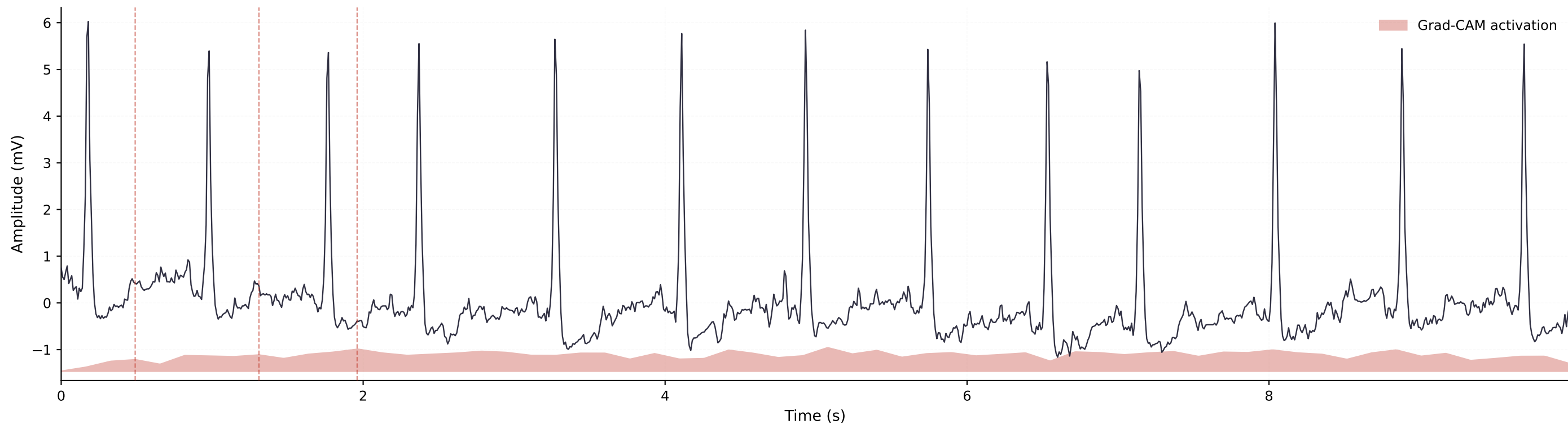
A Grad-CAM explanation — LVH (Lead I)
