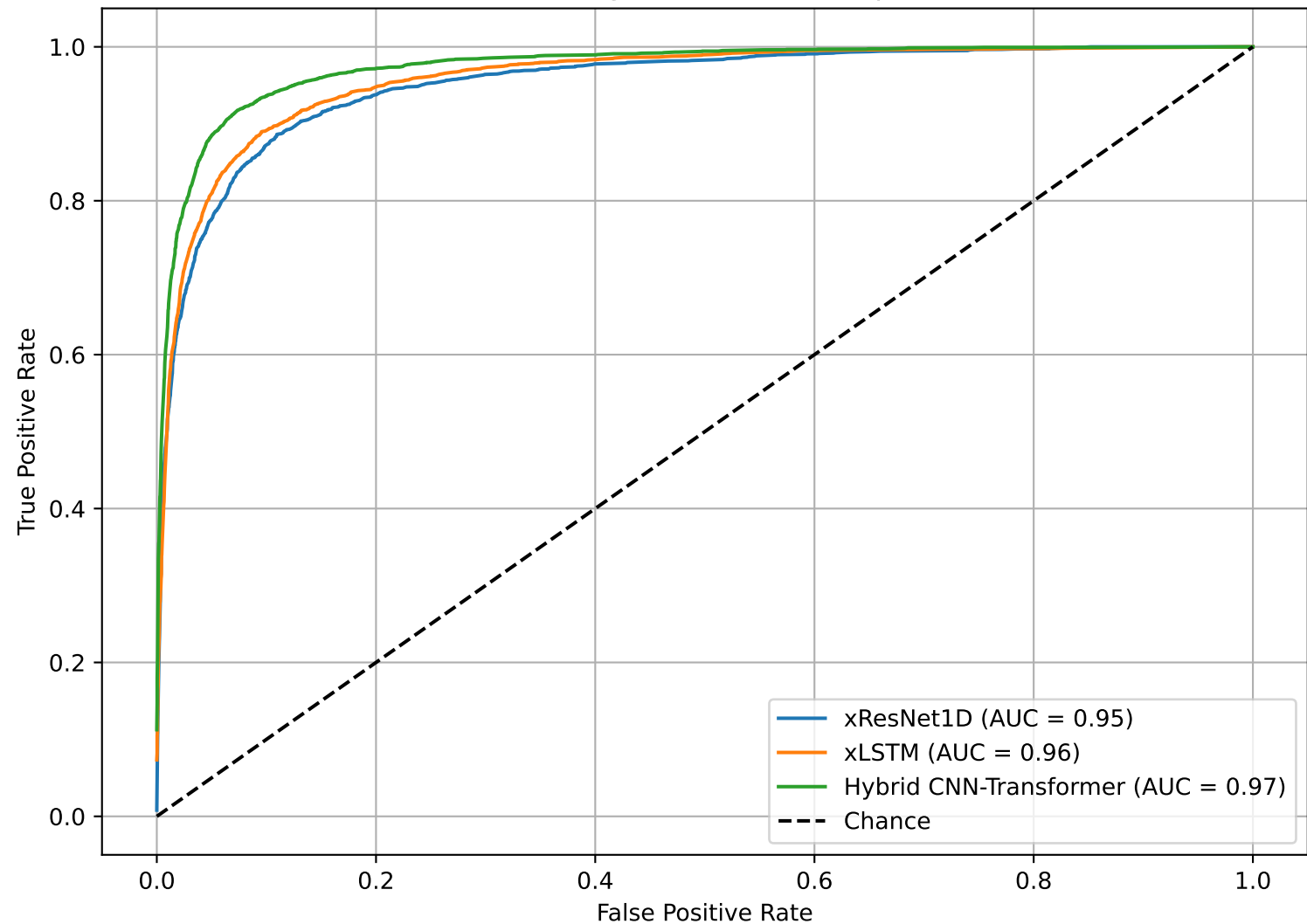
Macro-Average ROC Curve Comparison
