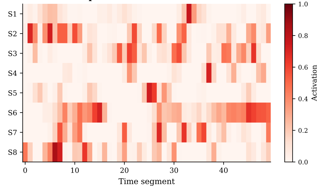
C Cross-sample activation — AFIB
