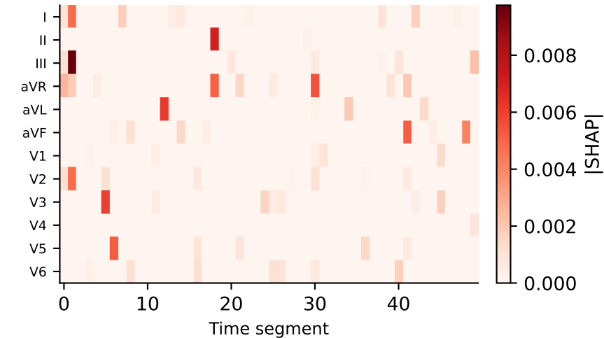
C SHAP heatmap lead x time
