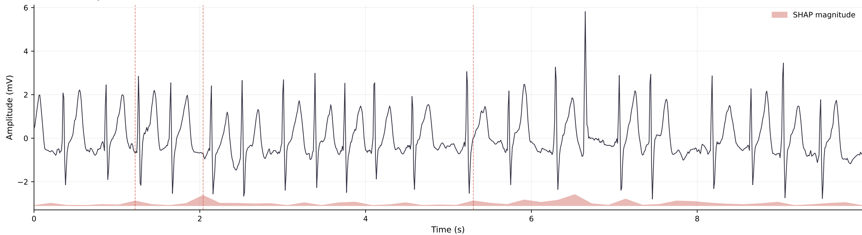
A SHAP explanation — AFIB (Lead I)
