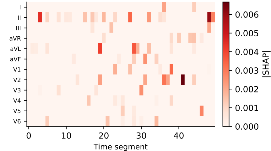
C SHAP heatmap lead × time
