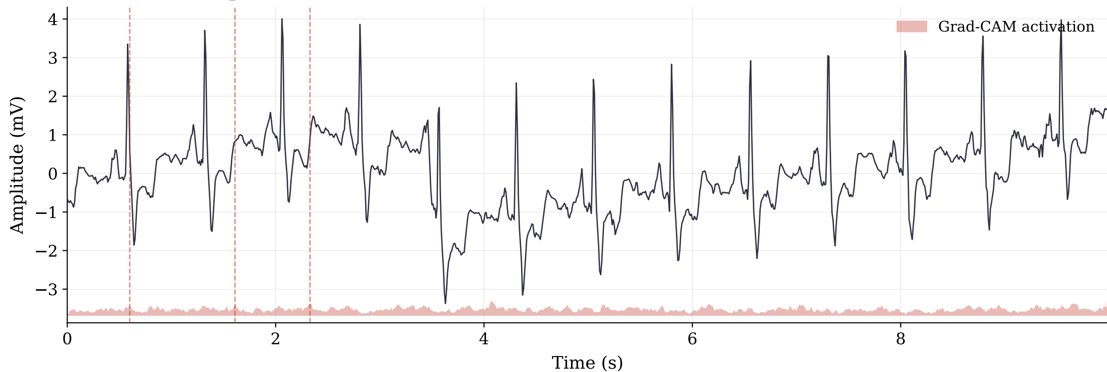
A Grad-CAM Explanation — LAFB (Lead I)
