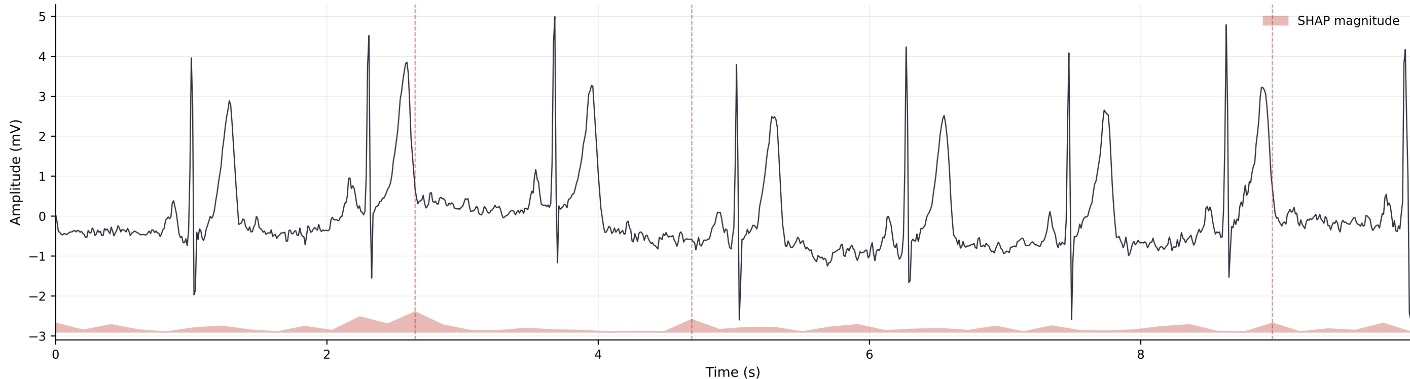
A SHAP explanation — NORM (Lead I)
