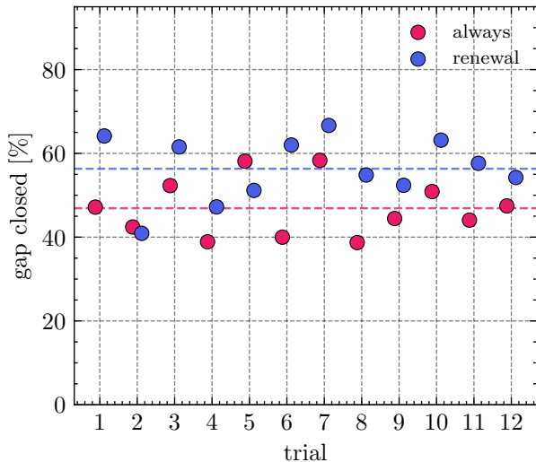
iid Bernoulli ( p_{\text{clear}} = 0.34 )
