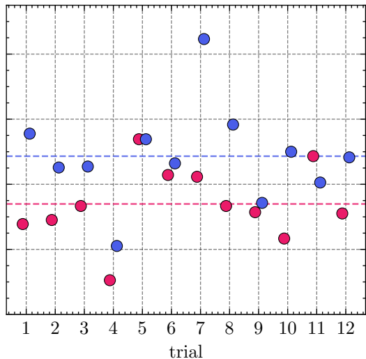
BCM (real cloud masks)
