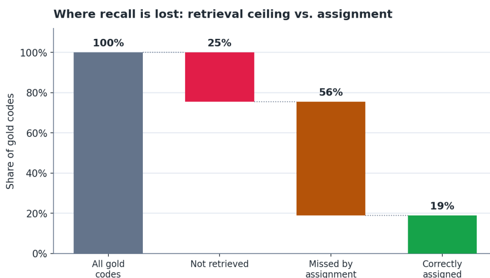
Figure 4 — Recall decomposition. The gap from 100% to the ceiling is what retrieval never surfaced; the gap from the ceiling to the green bar is what the assignment model lost. This tells you exactly where to invest next.
