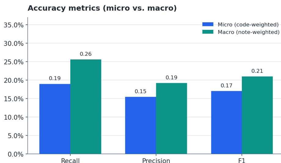
Figure 3 — Accuracy metrics, micro vs. macro.
