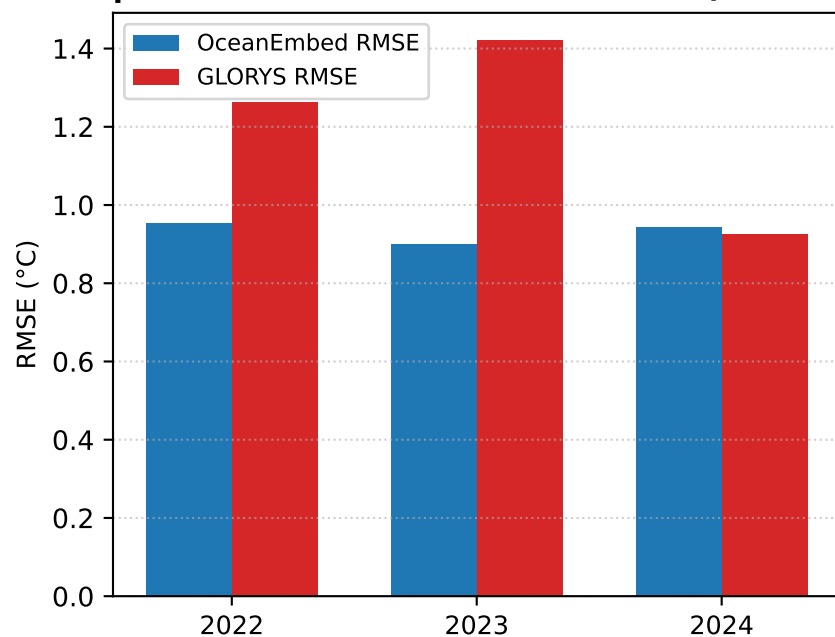
Temporal Generalization: Unseen Years (2022-2024)
