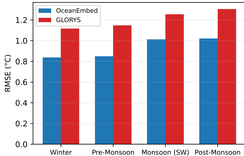
Seasonal Regime Breakdown
