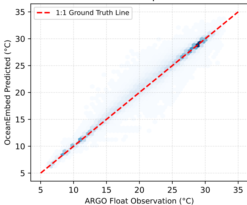
OceanEmbed vs In-Situ ARGO RMSE: 0.9336°C | R 2 : 0.9827
