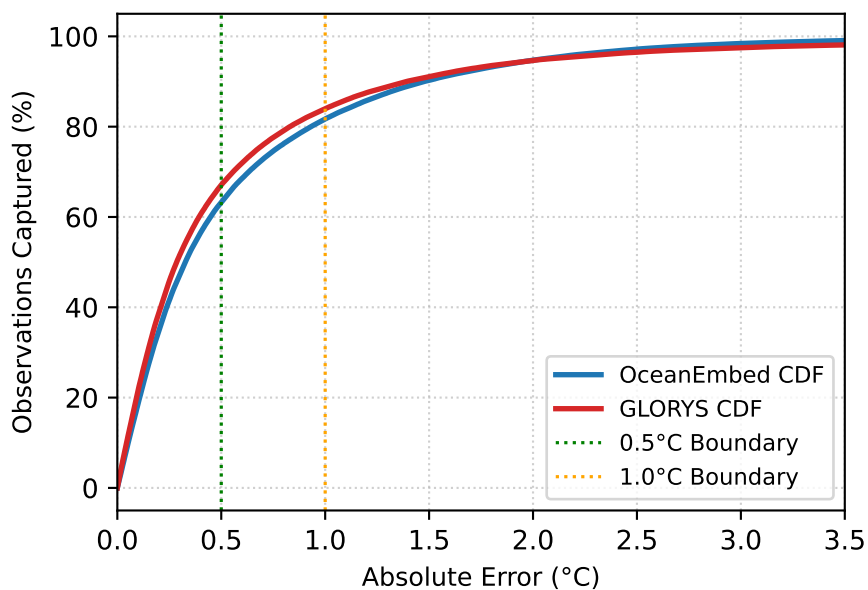
Cumulative Absolute Error Distribution
