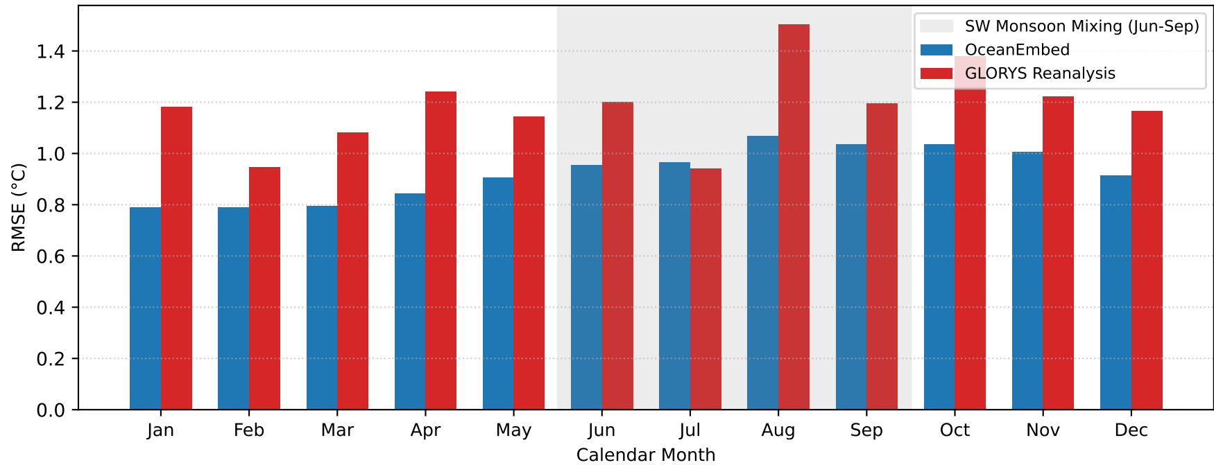
Month-by-Month Predictive Stability Across Diverse Hydrographic Regimes
