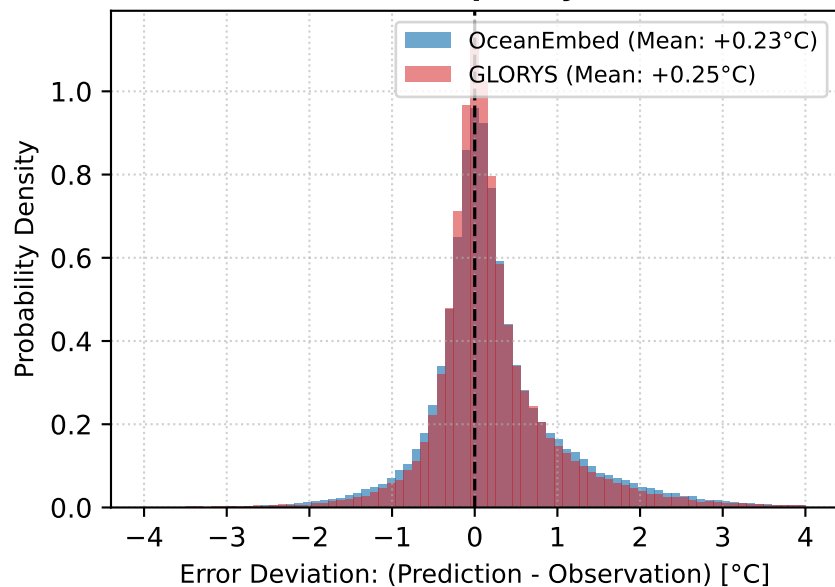
Residual Error Frequency Distribution
