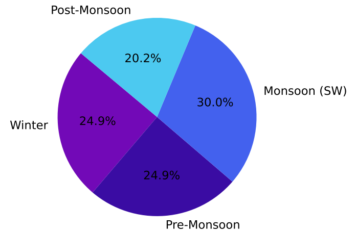
In-Situ Validation Profile Density by Season
