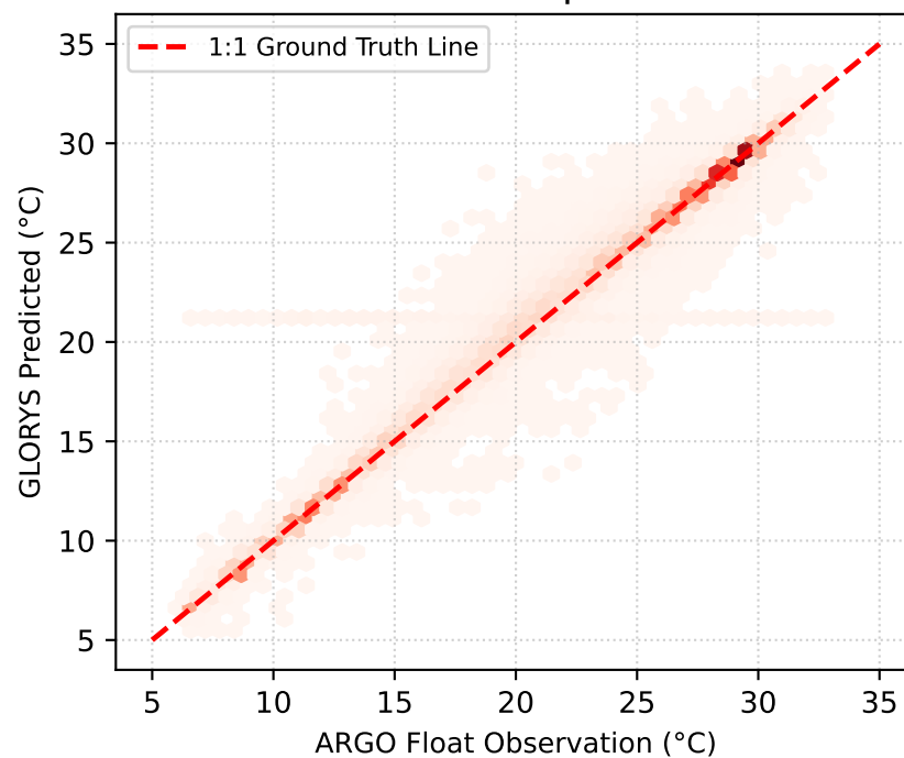
GLORYS12V1 vs In-Situ ARGO RMSE: 1.2059°C | R 2 : 0.9712
