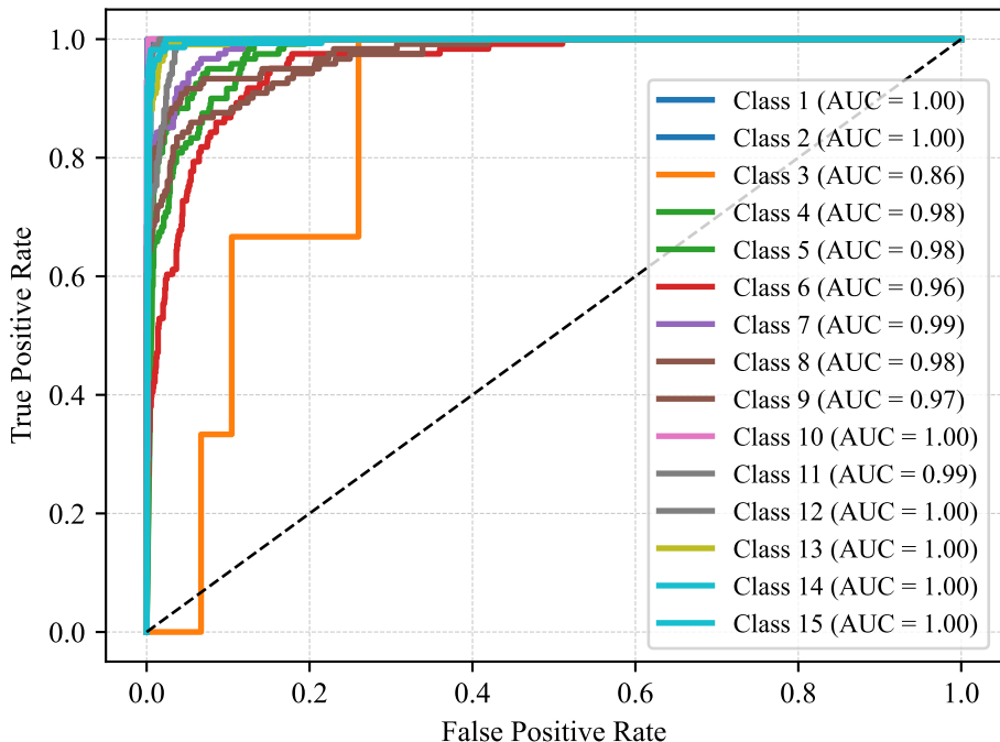
ROC Curve - Multiclass
