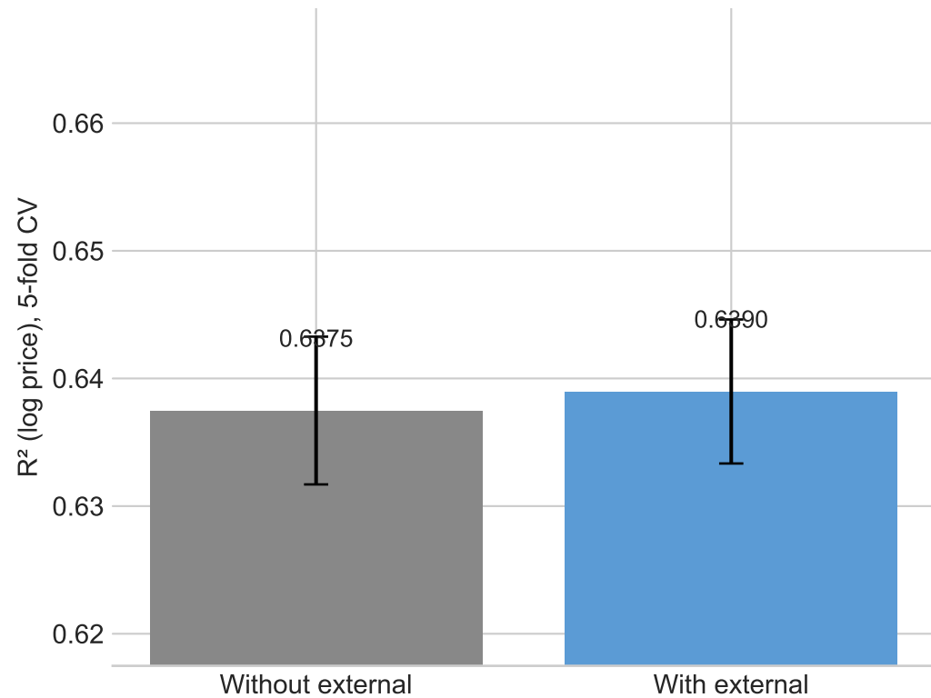
Stacked ensemble — CV R^2
