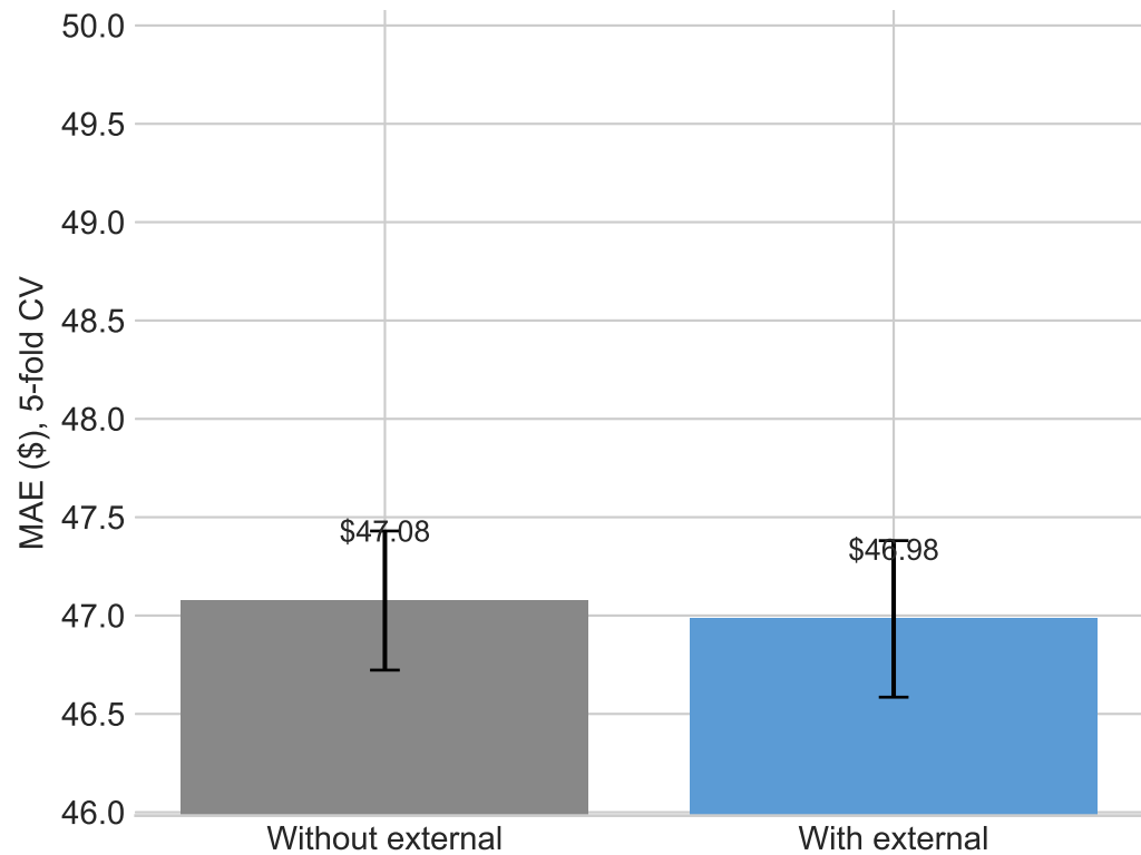
Stacked ensemble — CV MAE
