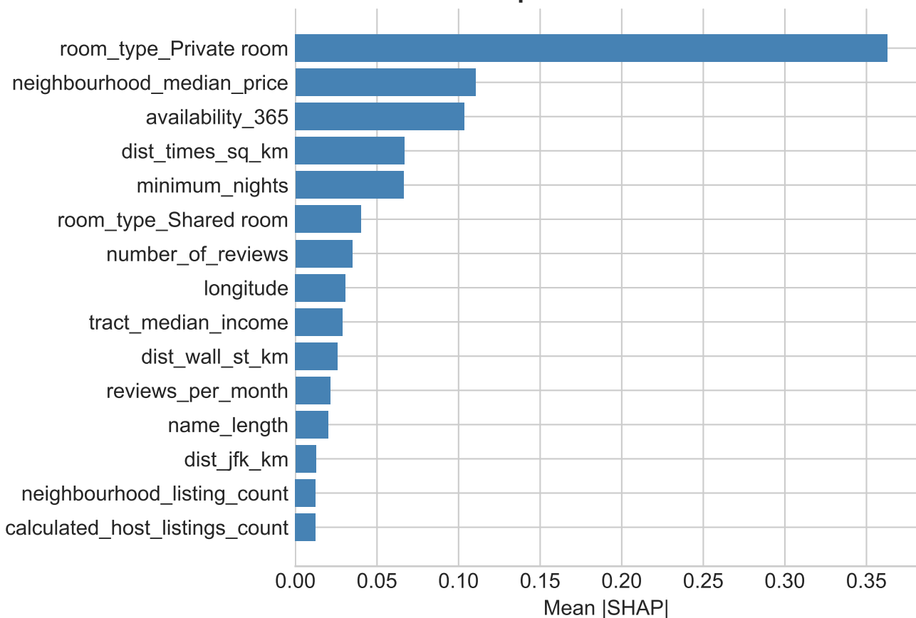
Feature importance — tuned HistGB
