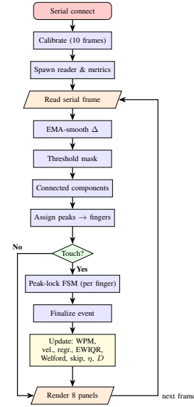
Fig. 3. Software pipeline: three-thread serial ingestion, dual-finger touch detection via connected-component analysis and per-finger peak-lock FSM, eight metric trackers implementing seven performance metrics ( D = composite difficulty score; EWIQ and Welford are sub-trackers of velocity-IQR and ToT respectively), and eight-panel live visualization.
