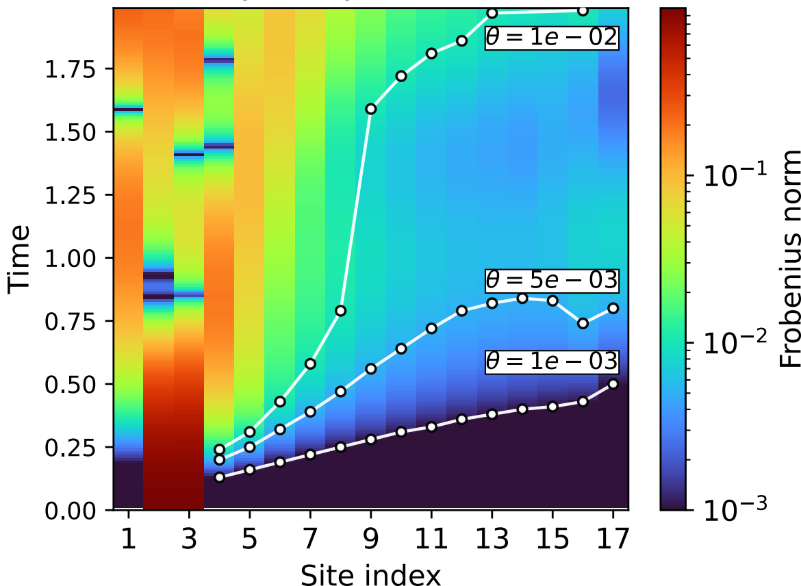
(2;3), J_z = 1, J_x = 20, \alpha = 0.9
