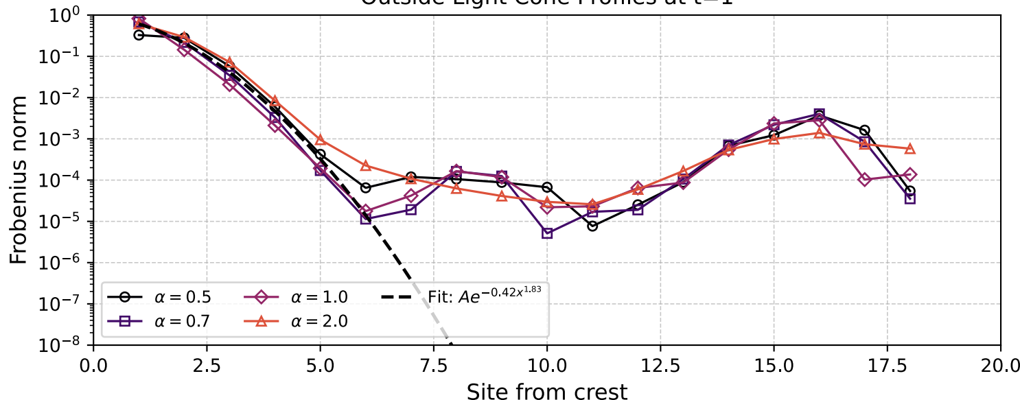
Outside Light Cone Profiles at t=1
