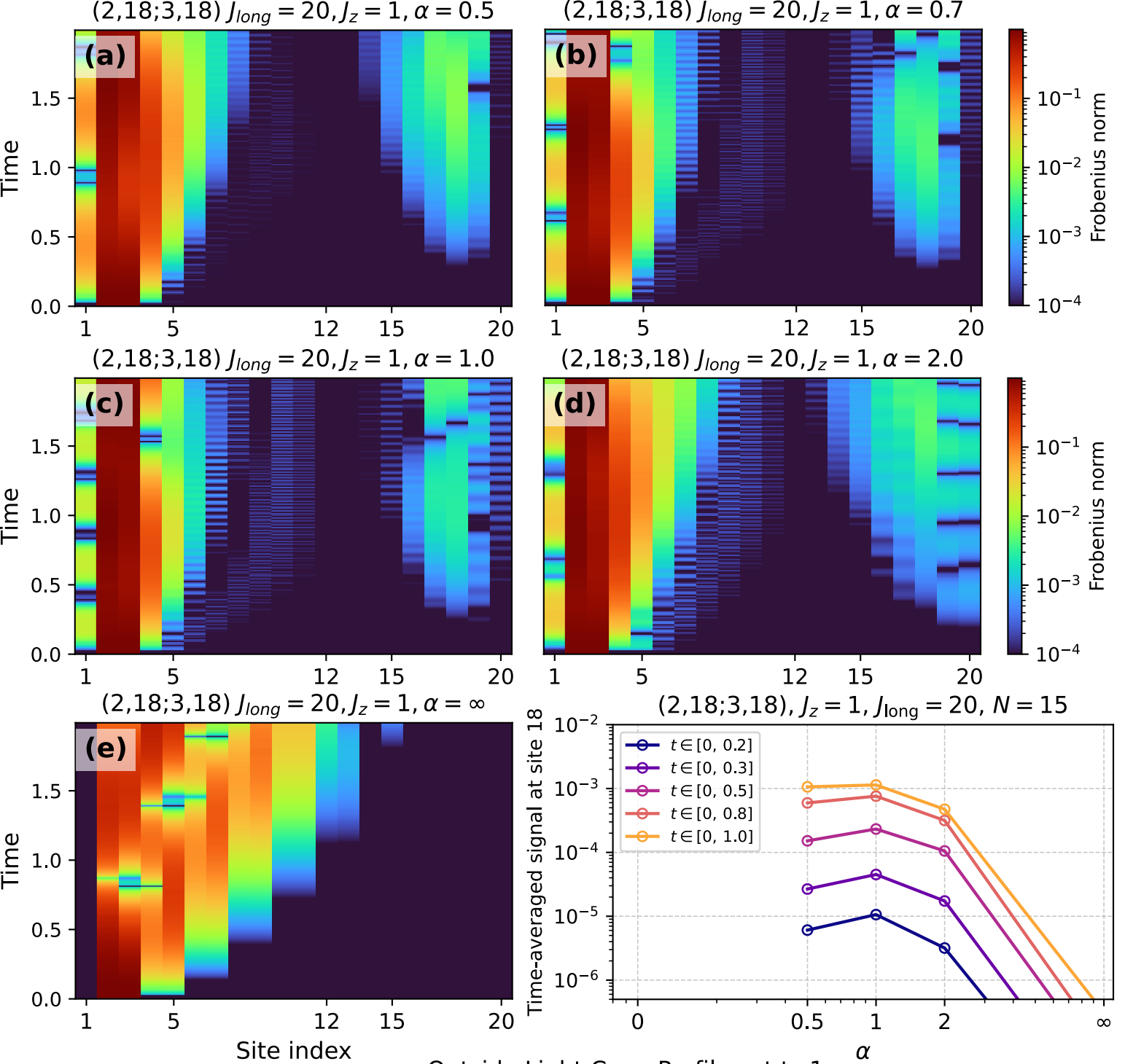
Outside Light Cone Profiles at t=1
