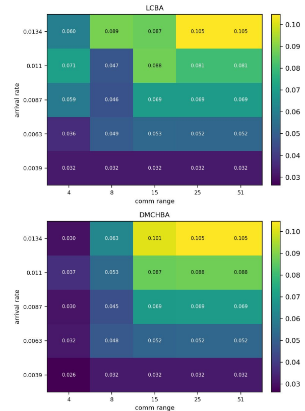
Figure: Steady-State Throughput — Warehouse Small (30×30, 6 agents)
