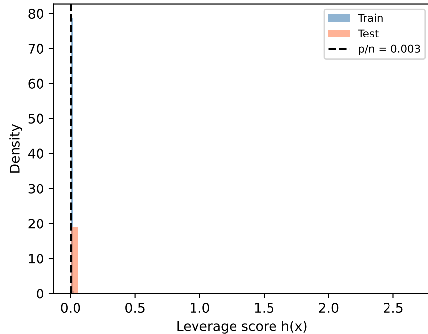
California (p=8, n=3000)
