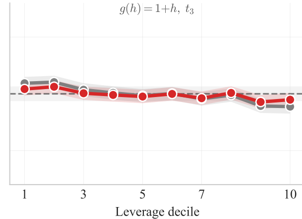
Heavy-tailed
