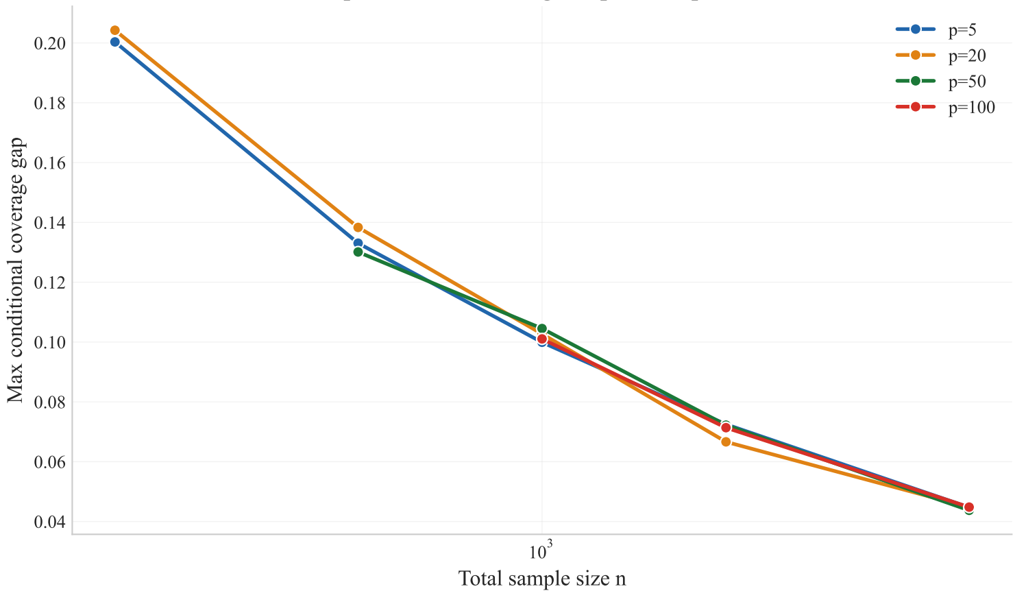
Experiment 9: Coverage Gap vs Sample Size
