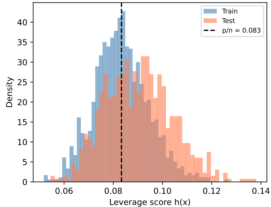
Sparse-HD (p=100, n=1200)
