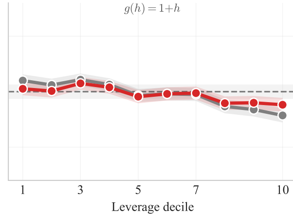
Textbook
