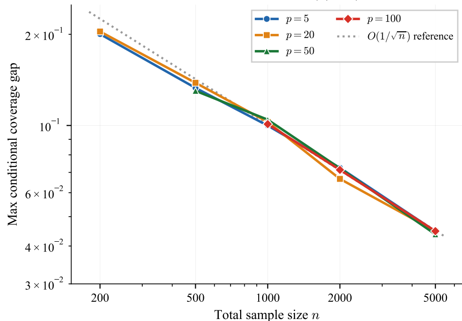
(b) Gap \rightarrow 0 at rate O(1/\sqrt{n})
