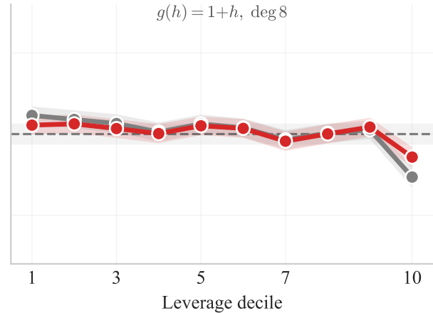
Polynomial
