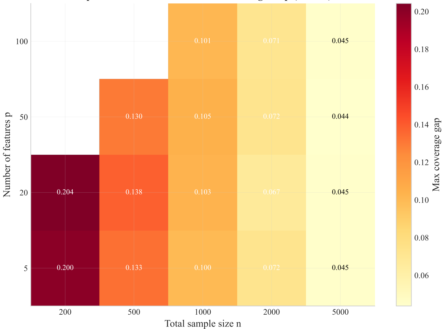
Experiment 9: Max Conditional Coverage Gap (LWCP)
