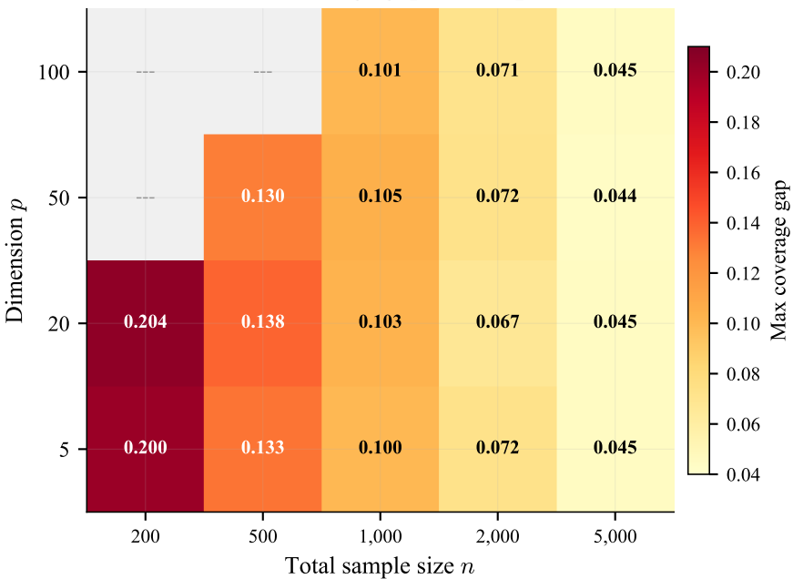
(a) Coverage gap heatmap
