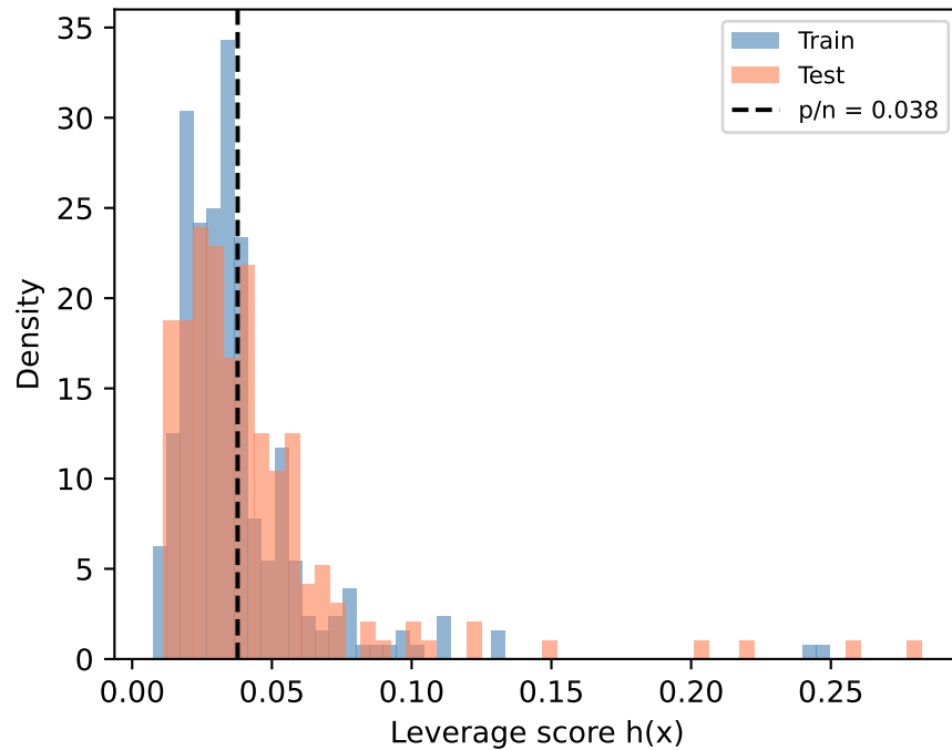
Diabetes (p=10, n=265)
