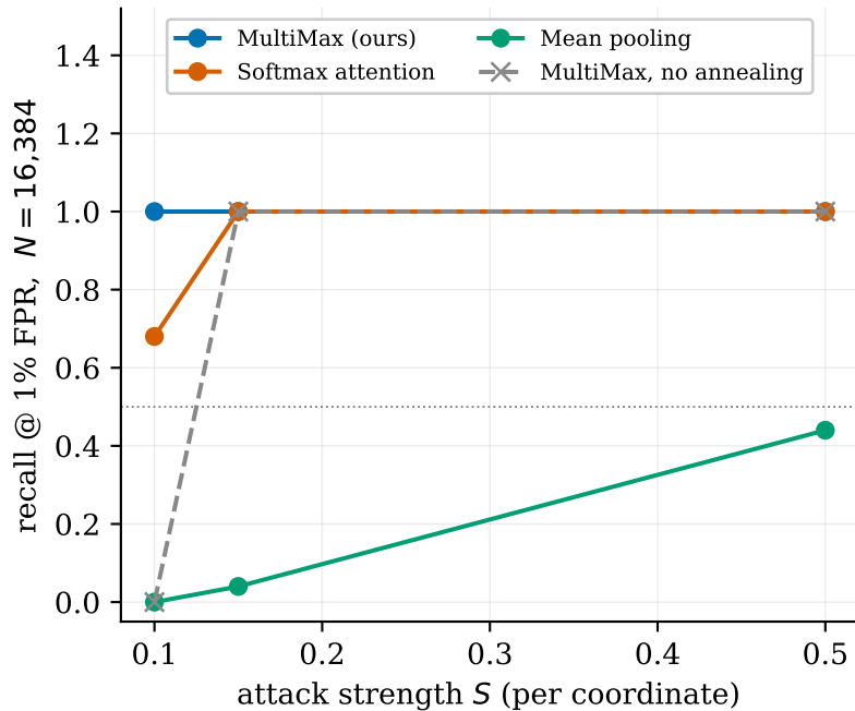
Weak-signal recall
