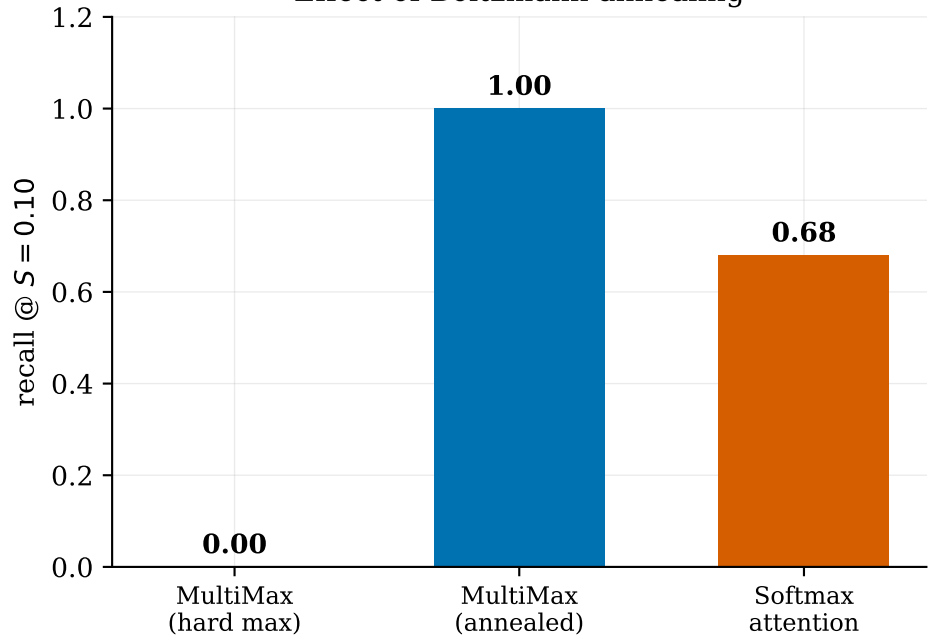
Effect of Boltzmann annealing
