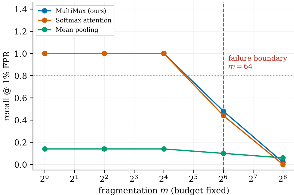
Detection under fragmentation
