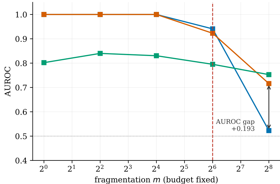
Ranking quality past the boundary
