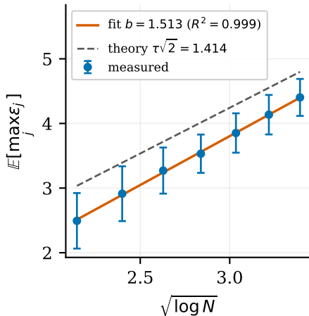
(b) benign-maximum drift
