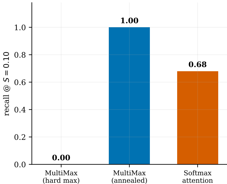
Effect of Boltzmann annealing
