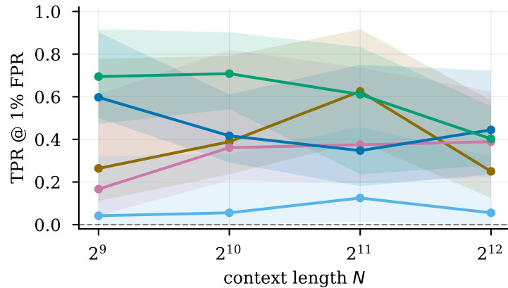
qwen2.5-7b: TPR @ 1% FPR vs length
