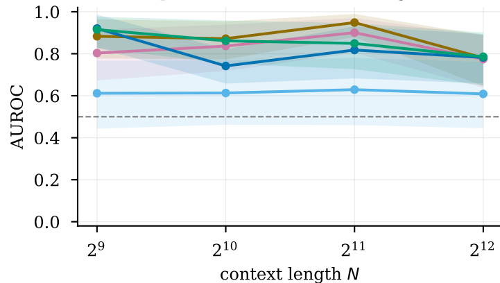
qwen2.5-7b: AUROC vs length
