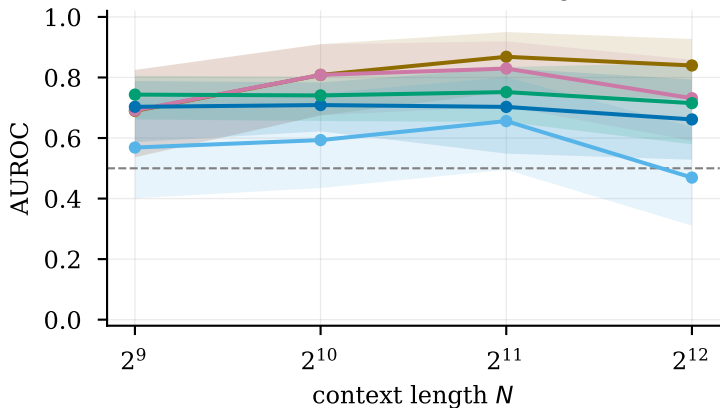
mistral-7b: AUROC vs length
