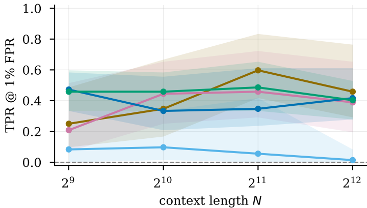
mistral-7b: TPR @ 1% FPR vs length
