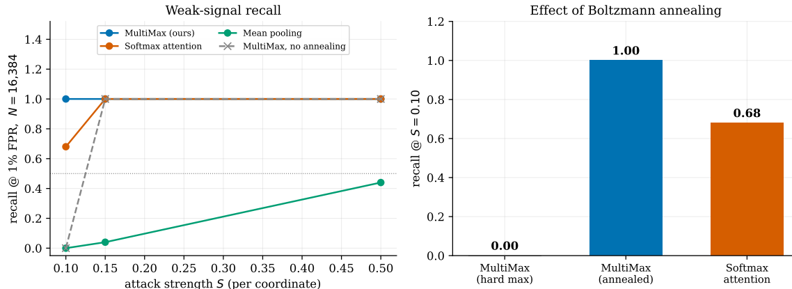
Figure 6: Recall at 1% FPR, N=16,384 , trained at N=512 . Annealing converts a total training failure at S=0.10 into full recall.
