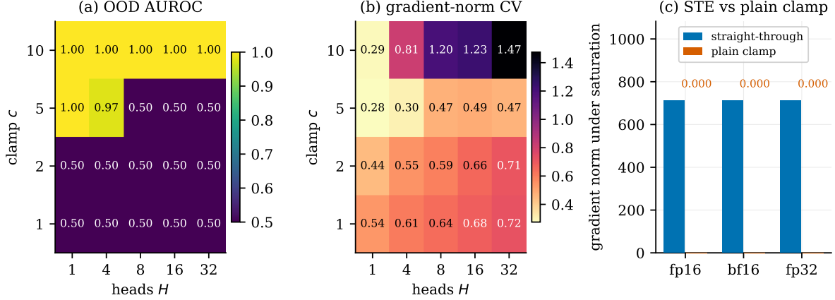
Figure 8: (a) Out-of-distribution AUROC over the c \times H grid: probes train at N=512 and are scored at N=16,384 . The usable region is a staircase, and the c required grows with H . (b) Coefficient of variation of the gradient norm across training, a scale-free stability measure comparable across H . (c) Gradient norm under deliberate saturation, by compute precision.
