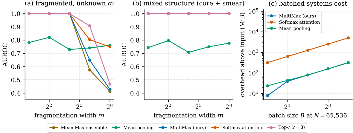
Figure 12: (a) AUROC against fragmentation width under an unknown- m protocol: probes train on a mixture m \in \{1, 8, 64\} and are evaluated at held-out widths. (b) The mixed adversary, which retains a concentrated core carrying half the budget. (c) Per-sequence overhead against batch size at N=65,536 .
