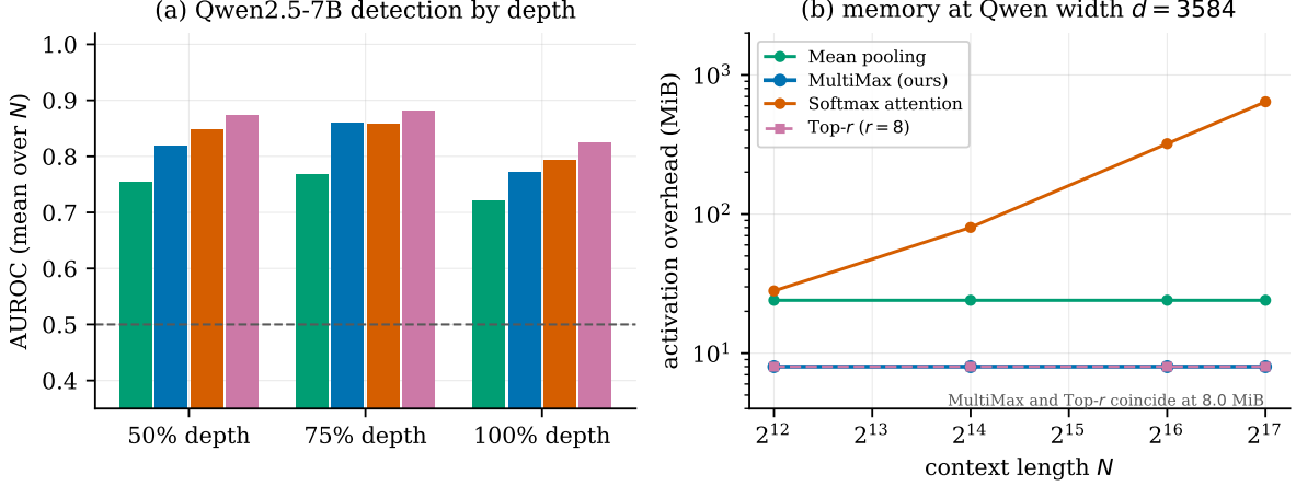
Figure 9: Qwen2.5-7B. (a) Detection AUROC by depth ratio, averaged over N \in \{256, 1024, 4096\} . (b) Activation overhead at Qwen’s width d=3584 : MultiMax and Top- r are flat at 8.0 MiB to N=131,072 while softmax pooling reaches 641.0 MiB.
