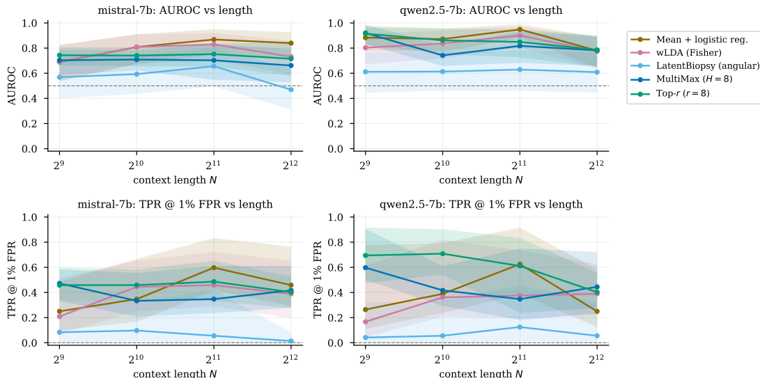
Figure 4: Both metrics against context length for both model families, averaged over depth, with 95% bootstrap intervals shaded. The ribbons overlap almost everywhere, which is the honest summary of a 24 + 24 evaluation; the one consistent separation is the angular baseline at the bottom of the lower row.
