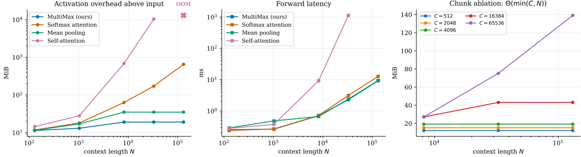
Figure 5: Left, centre: activation overhead above the input tensor, and forward latency, versus N . Right: the chunk ablation, in which rows are flat in N once chunking engages and columns rise with C .
