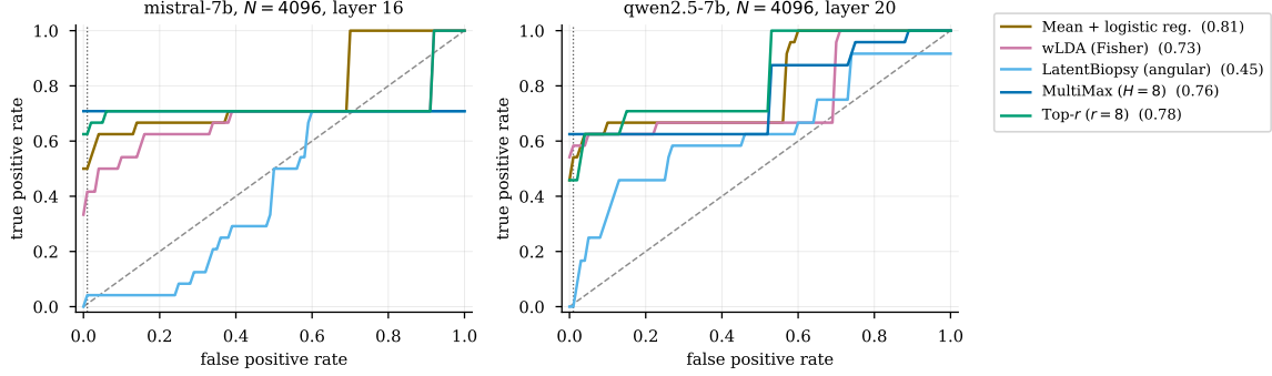
Figure 3: ROC at N=4096 against the two baseline families, at the depth where the aggregators perform best on each model. The dotted vertical line is the 1% FPR operating point. Areas in the legend are AUROC.
