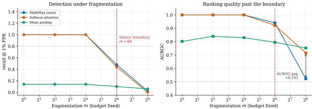
Figure 11: Fragmented attack: a fixed budget S=2.0 split across m non-contiguous tokens. Both pooled aggregators fail at m=64 ; past the boundary softmax retains markedly better ranking.
