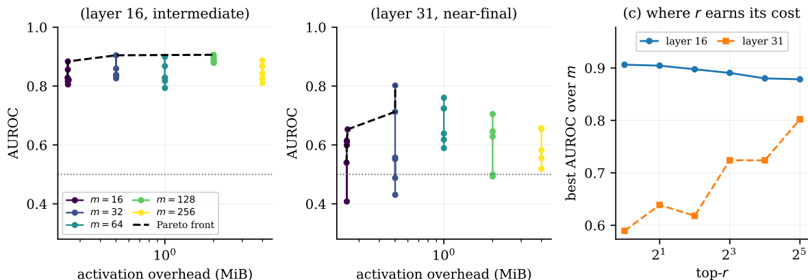
Figure 10: AUROC against activation overhead over the r \times m grid on real Mistral-7B residuals at N=1024 , needle-disjoint split, with the Pareto front dashed. Panel (c) isolates the effect of r : at the intermediate layer it buys nothing, and near the final layer it is worth 0.20 AUROC.
