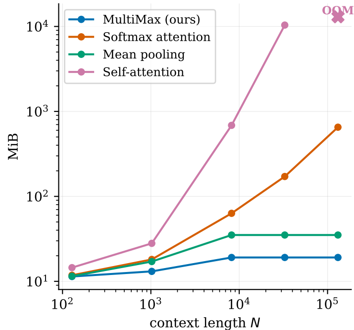
Activation overhead above input
