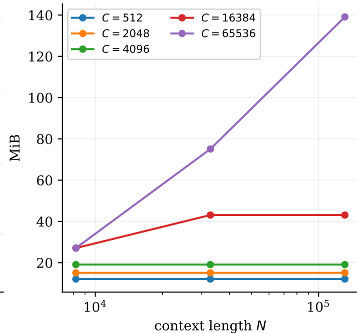
Chunk ablation: \Theta(\min(C, N))
