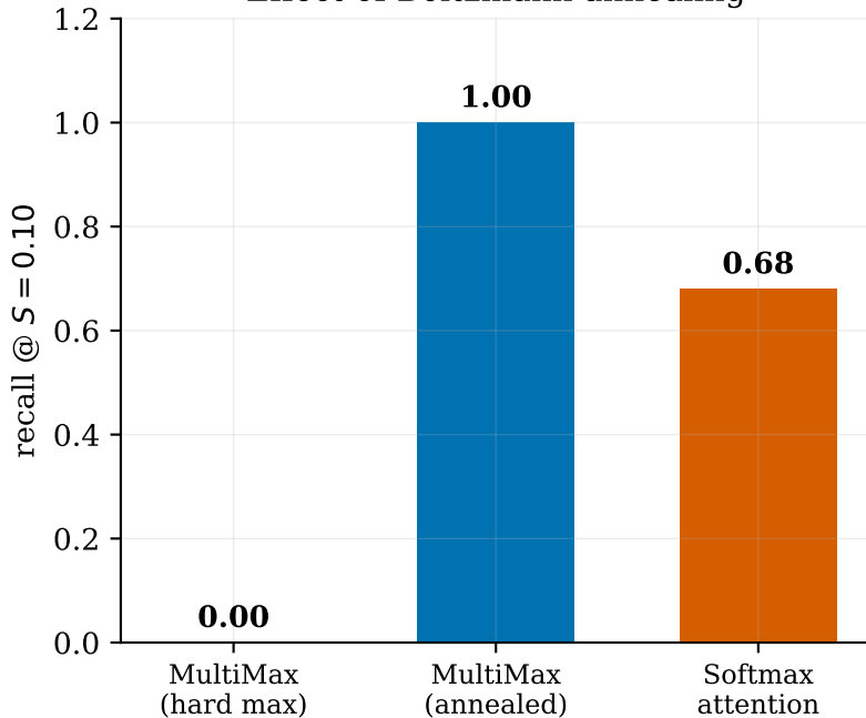
Effect of Boltzmann annealing
