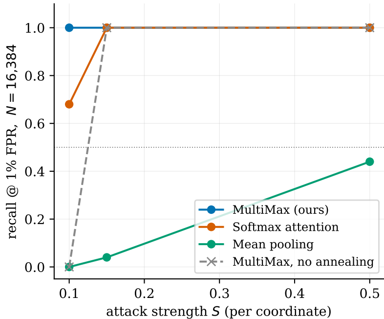
Weak-signal recall
