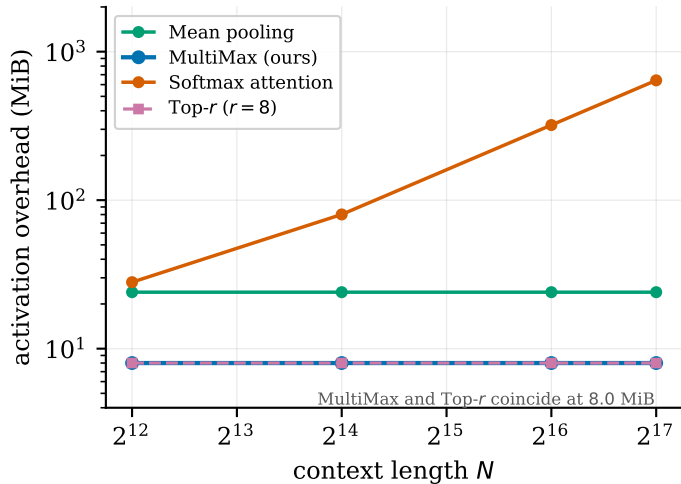
(b) memory at Qwen width d = 3584
