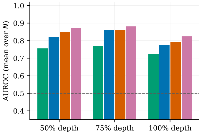
(a) Qwen2.5-7B detection by depth
