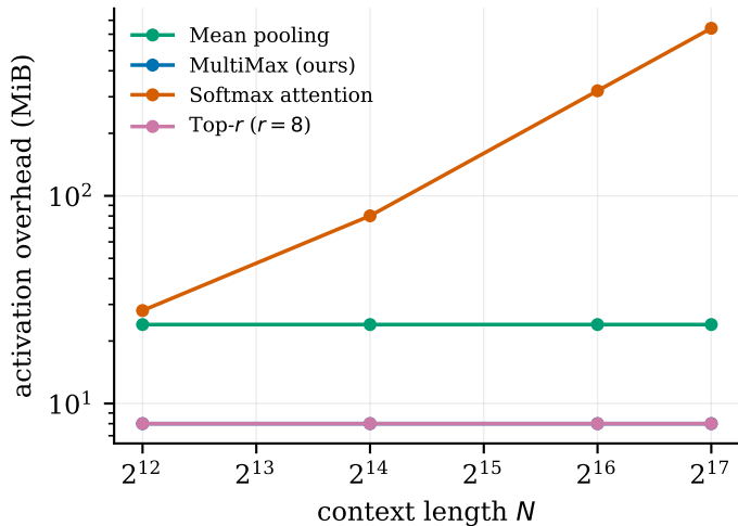
(b) memory at Qwen width d = 3584
