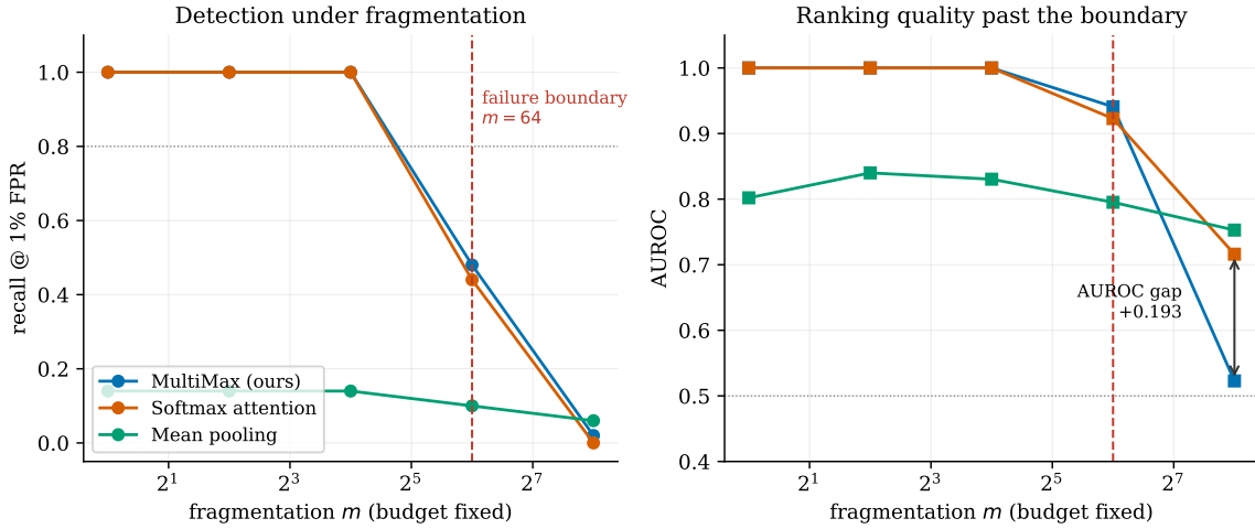
Figure 9: Fragmented attack: a fixed budget S=2.0 split across m non-contiguous tokens. Both pooled aggregators fail at m=64 ; past the boundary softmax retains markedly better ranking.
