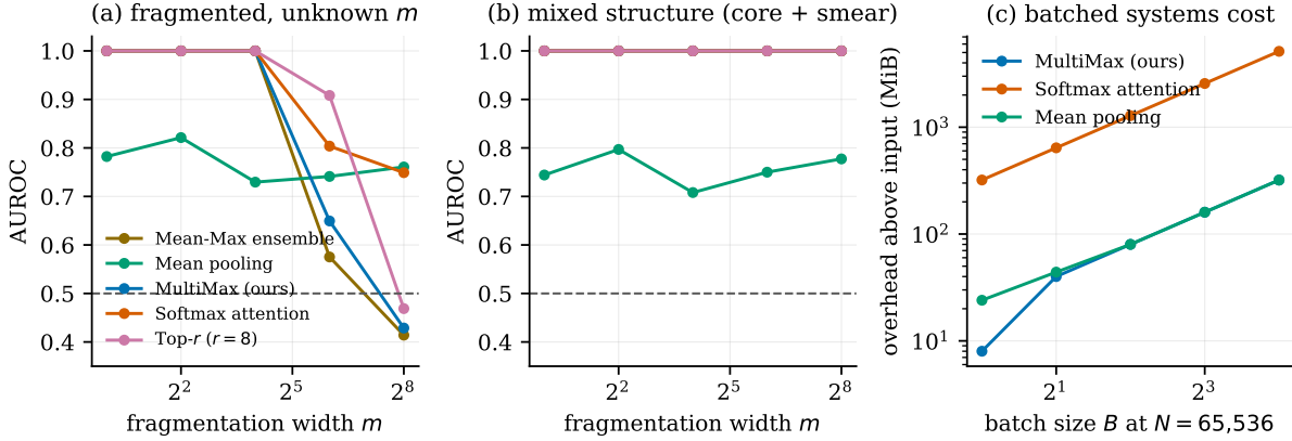
Figure 10: (a) AUROC against fragmentation width under an unknown- m protocol: probes train on a mixture m \in \{1, 8, 64\} and are evaluated at held-out widths. (b) The mixed adversary, which retains a concentrated core carrying half the budget. (c) Per-sequence overhead against batch size at N=65,536 .
