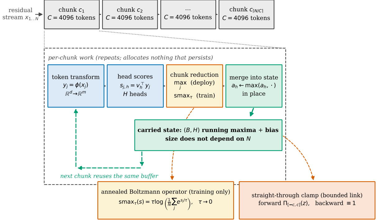
Figure 1: The streaming MultiMax pipeline. Chunks of C tokens enter one at a time; the token transform \phi and the head projection are applied within a chunk and discarded, and the only quantity that crosses a chunk boundary is the (B, H) buffer of running maxima. Its size is set by H , not by N , which is the whole of the memory claim. The two boxes at the foot are training-time mechanisms that leave the deployed map unchanged: the 1/N inside the Boltzmann operator of (9) removes an H\tau \log N length-dependent offset that plain LogSumExp would introduce (Remark 3.3), and the straight-through clamp keeps gradients alive in the saturated regime where a plain clamp returns exactly zero (Remark 2.1).
