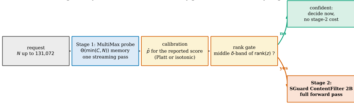
Two-stage safety cascade: a constant-memory gate in front of a heavyweight monitor
