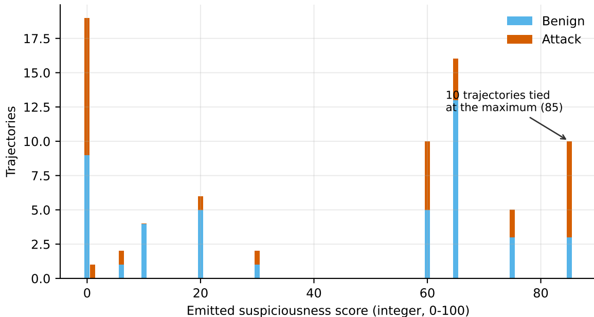
Figure 1. Distribution of the monitor's emitted integer score, stacked by true label. The score concentrates on a handful of round values, so a large block of trajectories is tied at the top and cannot be ranked against each other -- the regime where a small audit budget is spent.
