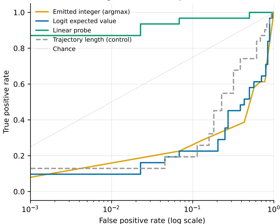
ROC with a log FPR axis, to expose the audit tail
