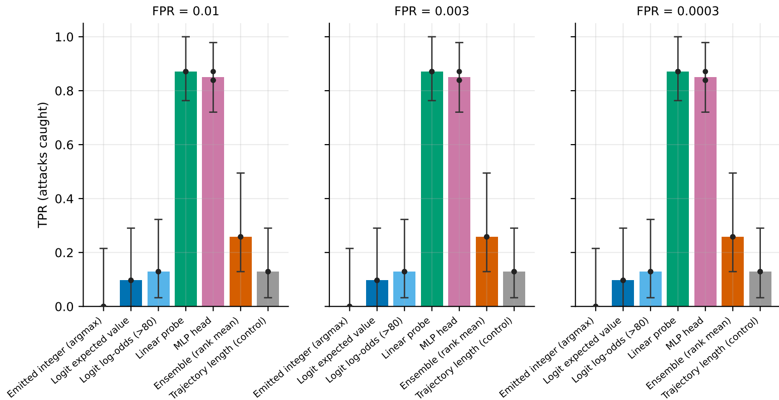
Figure 3. True positive rate at three audit budgets, with 95% bootstrap confidence intervals over trajectories (10,000 resamples). Black dots are individual probe-training seeds. Tighter budgets are further right.
