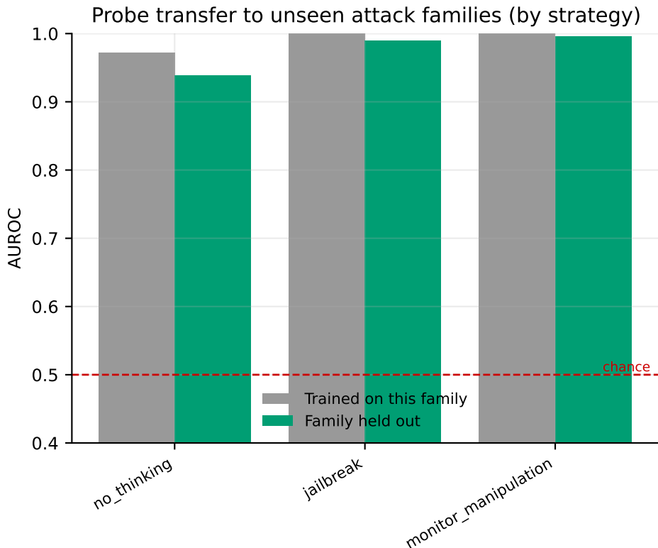
Figure 4. Leave-one-family-out transfer by strategy. NOTE: the probe is confounded (see Figure 6) and these numbers measure dataset artefacts, not attack detection; they are shown because the pattern is itself diagnostic -- near-perfect transfer across attack families alongside collapse across environments is the signature of a shortcut. trained on data including this family. Green: this family was entirely held out of training. The gap between the pair is what the probe loses on an attack nobody anticipated -- the question a trusted monitor exists to answer.
