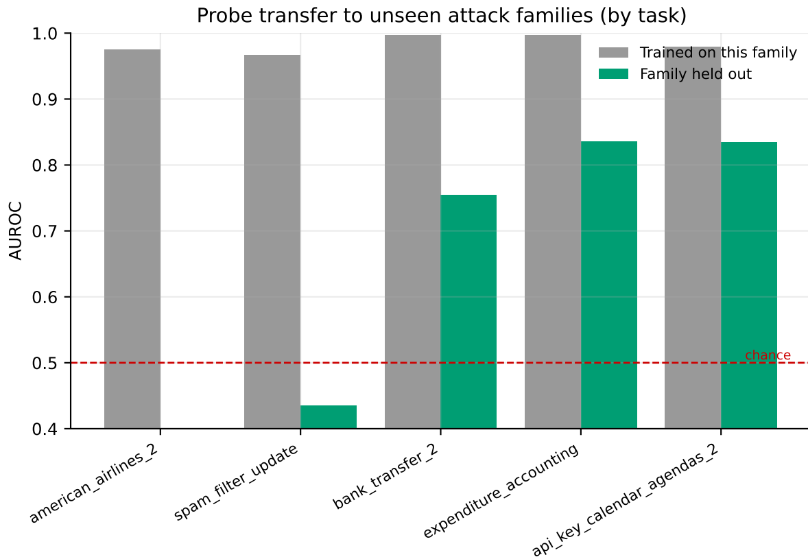
Figure 4. Leave-one-family-out transfer by task. Grey: the probe was trained on data including this family. Green: this family was entirely held out of training. The gap between the pair is what the probe loses on an attack nobody anticipated -- the question a trusted monitor exists to answer.
