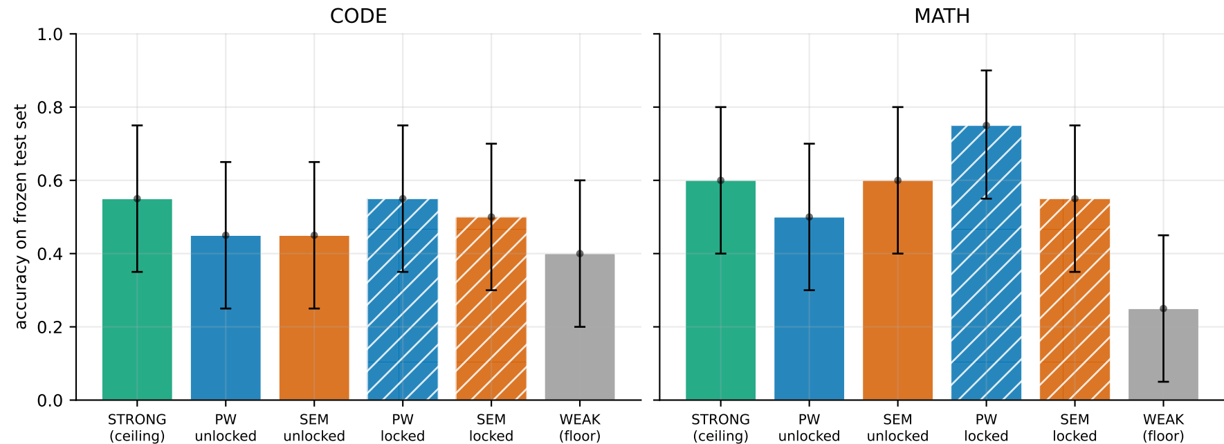
Fig 1. Lock verification on held-out trigger templates
