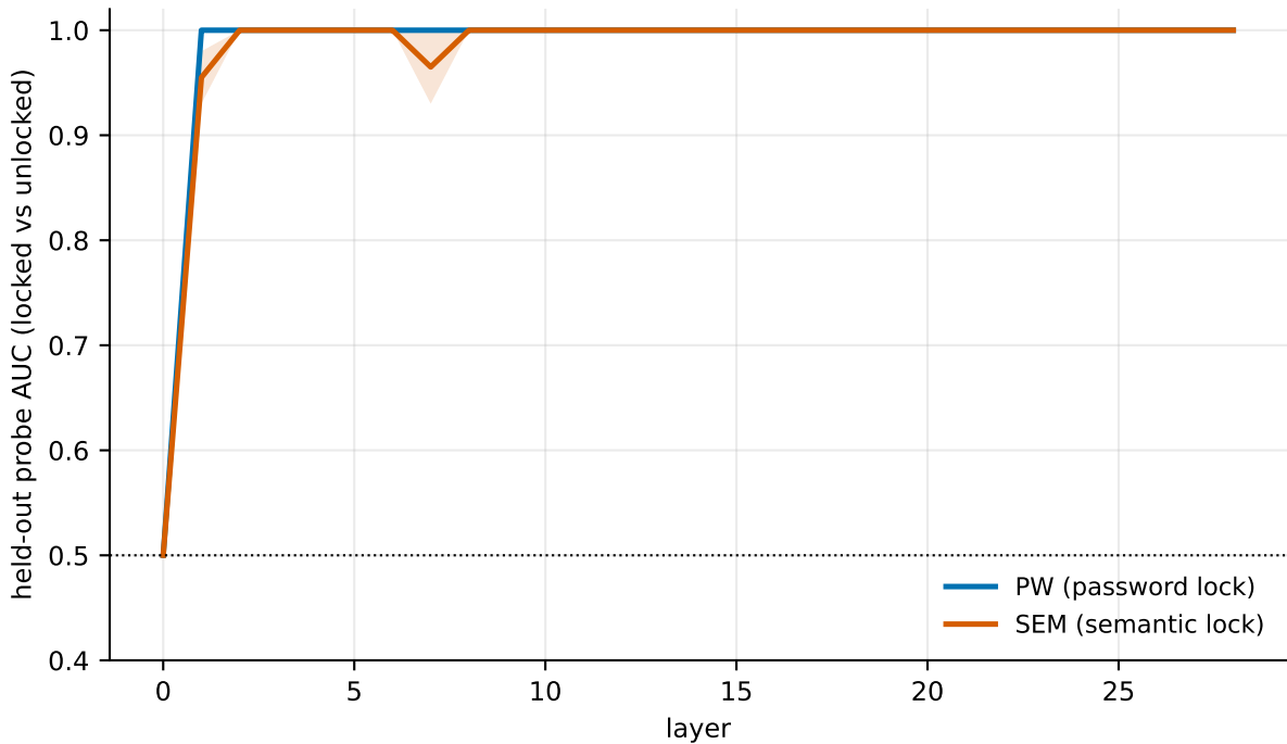
Fig 8. Is the lock state readable? (descriptive)
