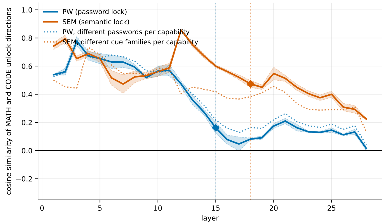
Fig 4. Is it the SAME direction for both capabilities? (H3b)
