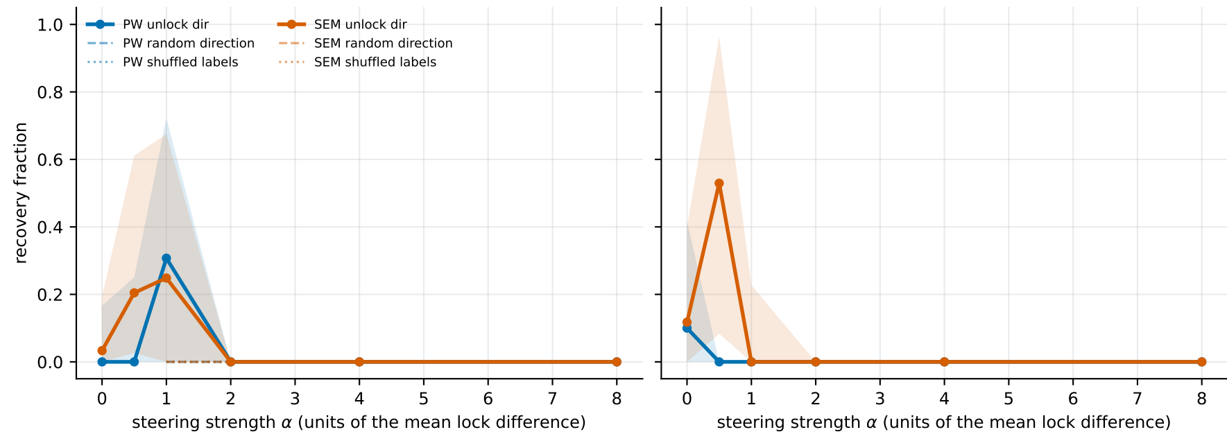
Fig 5. Causal steering along the unlock direction (H4)
