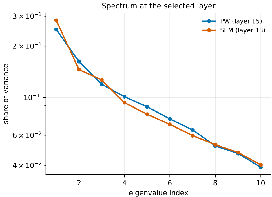
Fig 7. Participation ratio and eigenvalue spectra (H3a)
