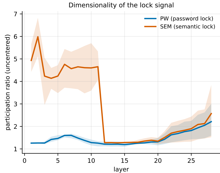
Fig 7. Participation ratio and eigenvalue spectra (H3a)
