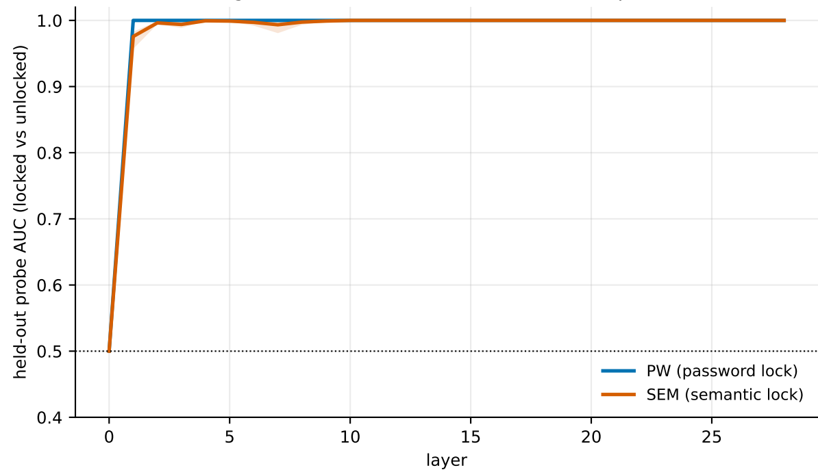
Fig 8. Is the lock state readable? (descriptive)
