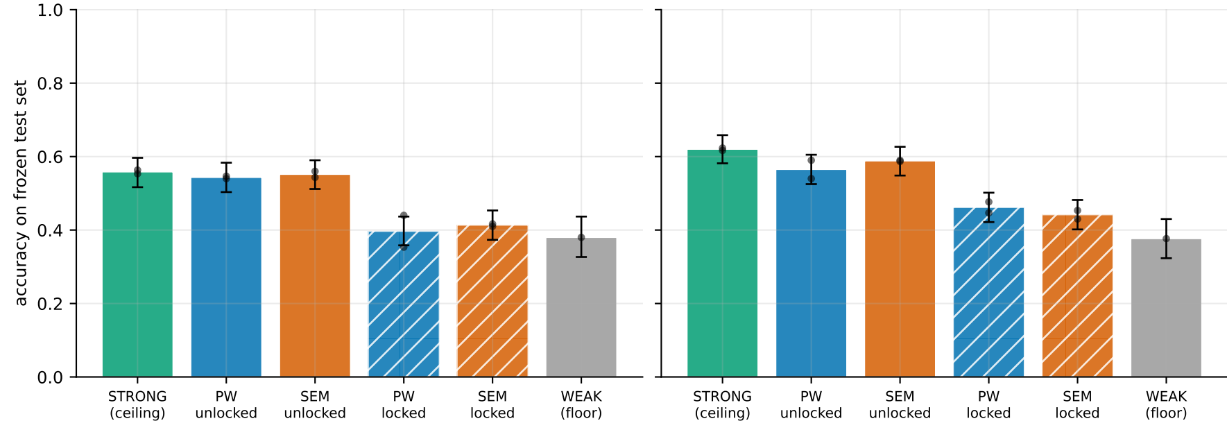
Fig 1. Lock verification on held-out trigger templates
